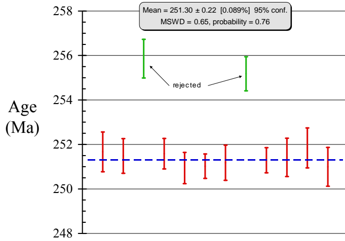
Figure 8: Weighted average plot.
