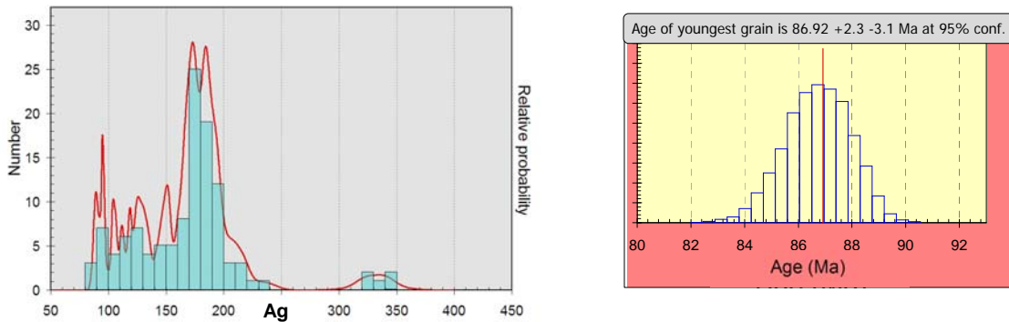
Figure 11: Left: Distribution of dates for a suite of detrital zircons. Right: Isoplot's output for youngest detrital grain. Vertical red line shows mode, blue boxes show distribution of Monte Carlo simulations.
