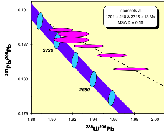
Figure 2: Tera-Wasserburg concordia plot (same data as Fig. 2).
